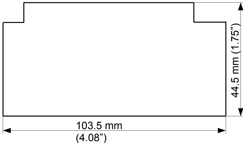
Fig. 1 Dimensions of GPS123D
